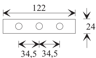
Mounting bracket Holes: 3 x Ø11.0 mm
