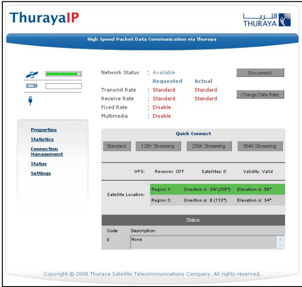
Home Screen
