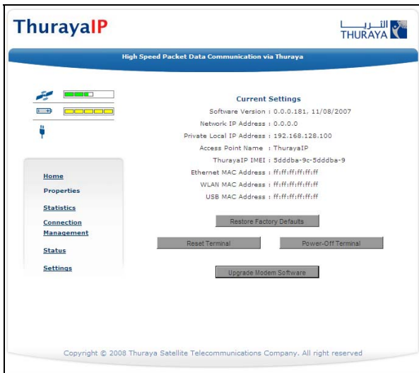
Properties Screen
