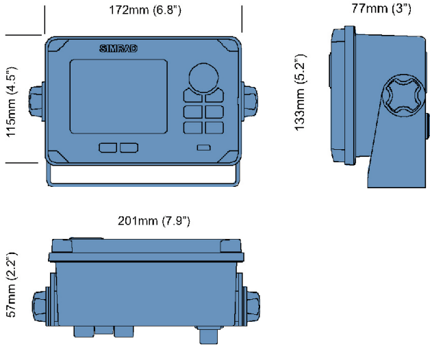
Figure 9.1 - AI50 dimensions
