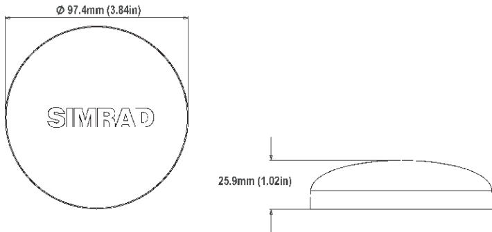
Figure 9.2 - Simrad GPS6 Antenna dimensions
