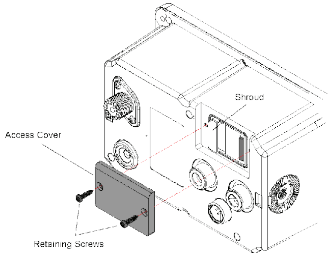
Figure. 2.5 - SD Card Access Cover
