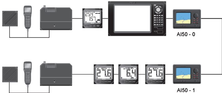
Figure 6.24 – Device Instance
